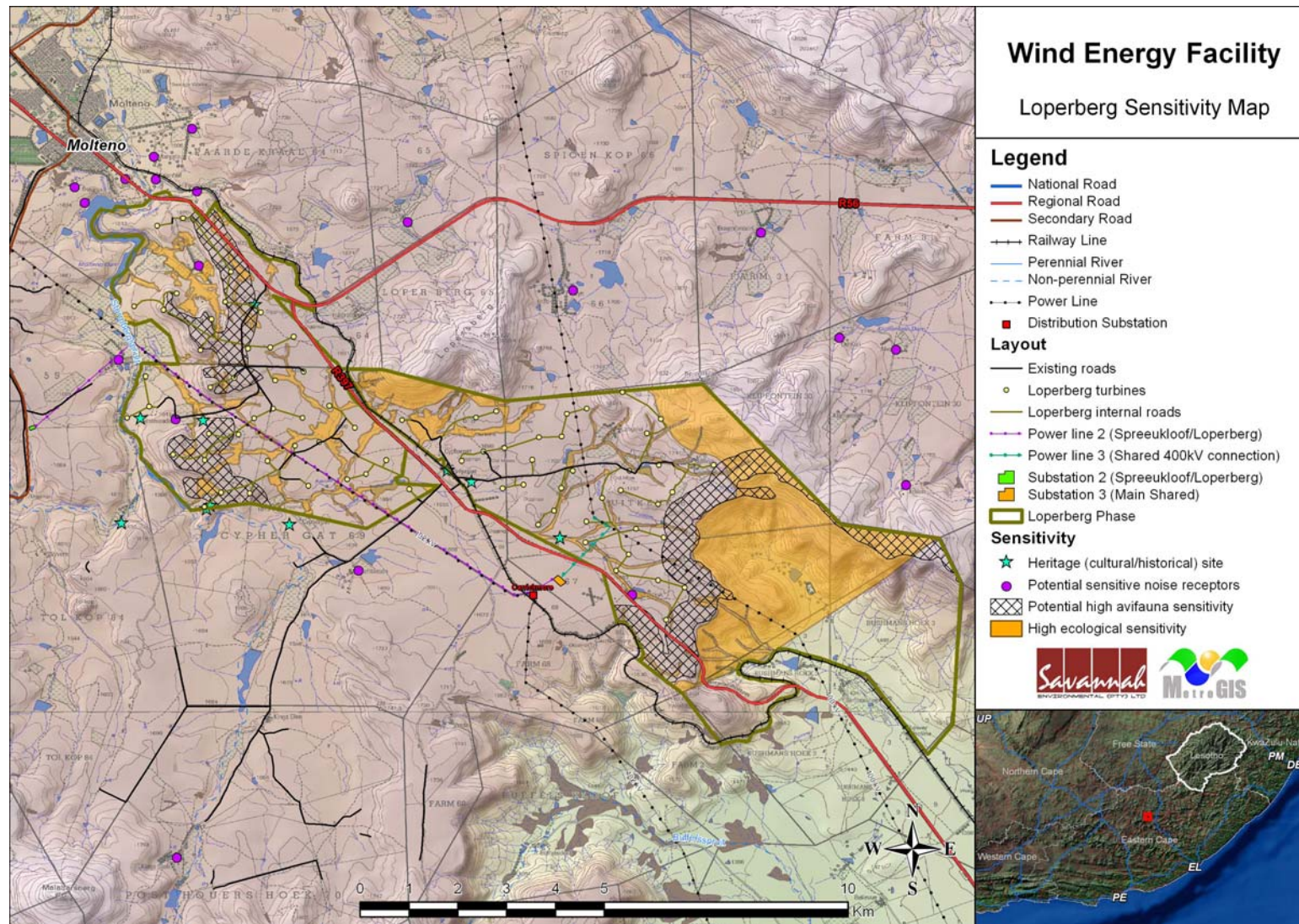
Figure 12.2: Combined sensitivity map for the Loperberg Wind Energy Facility project study area illustrating identified potentially sensitive areas in relation to the wind energy facility layout
