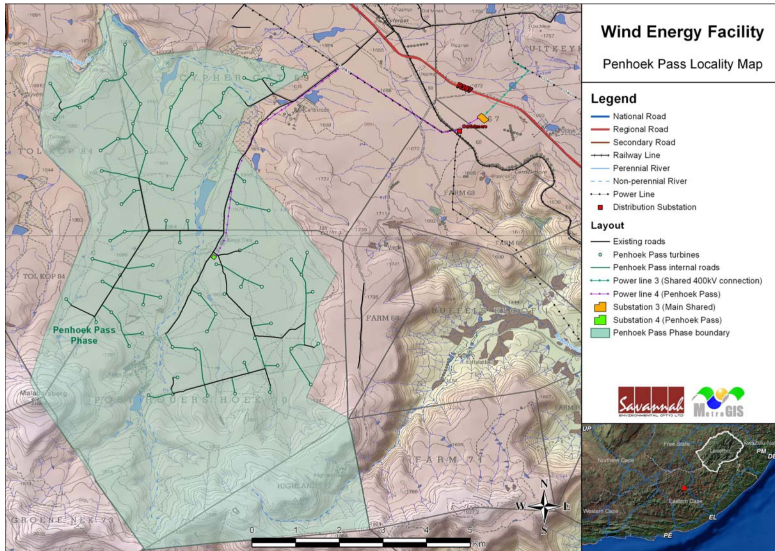
Figure 13.1: Map showing the proposed wind turbine layout, power line corridors and proposed substation sites for the Penhoek Pass Wind Energy Facility
