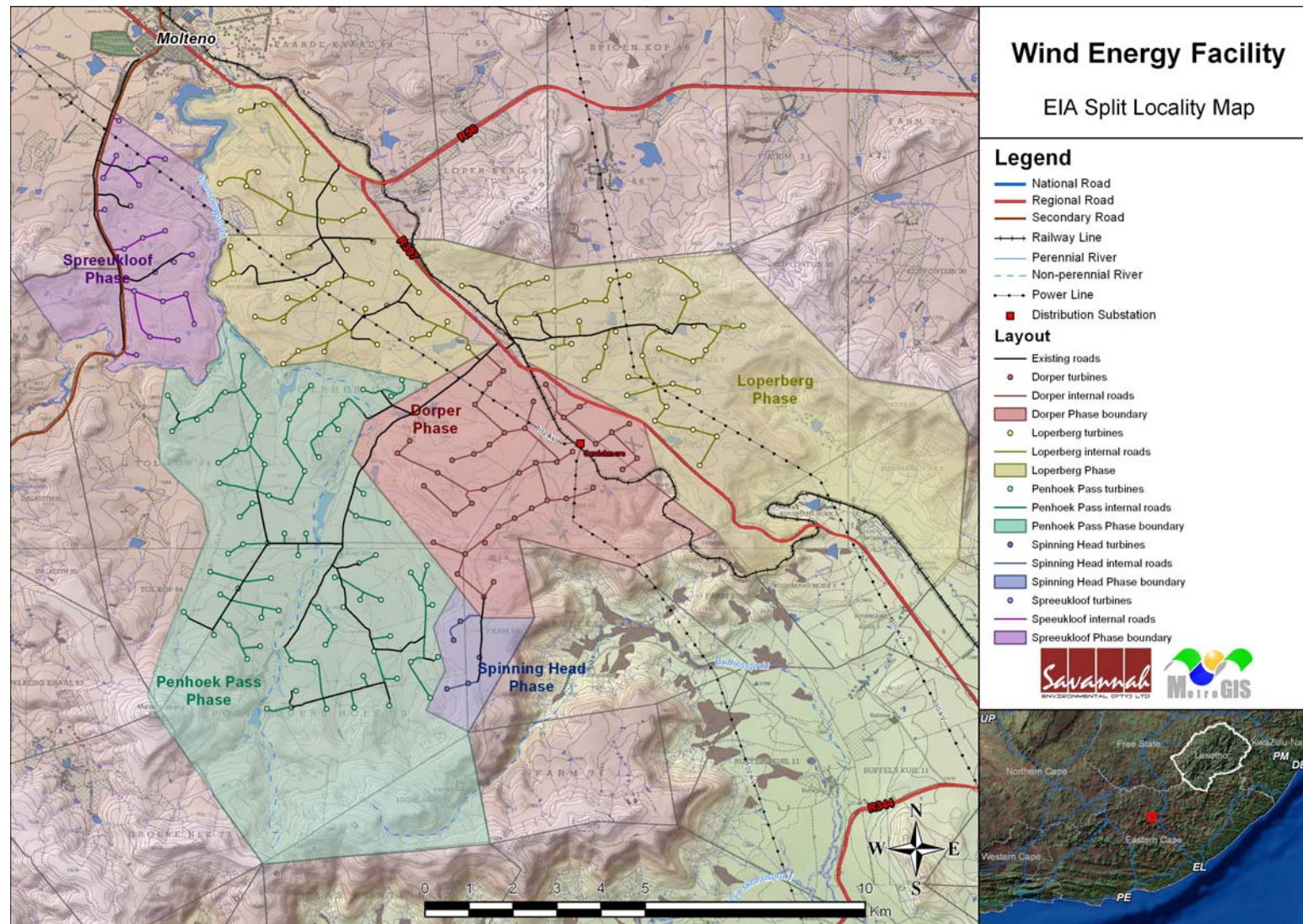
Figure 2.2: Locality map showing the properties included in the development site, as well as a provisional wind turbine layout, power line corridors and proposed substation locations within the development footprint
