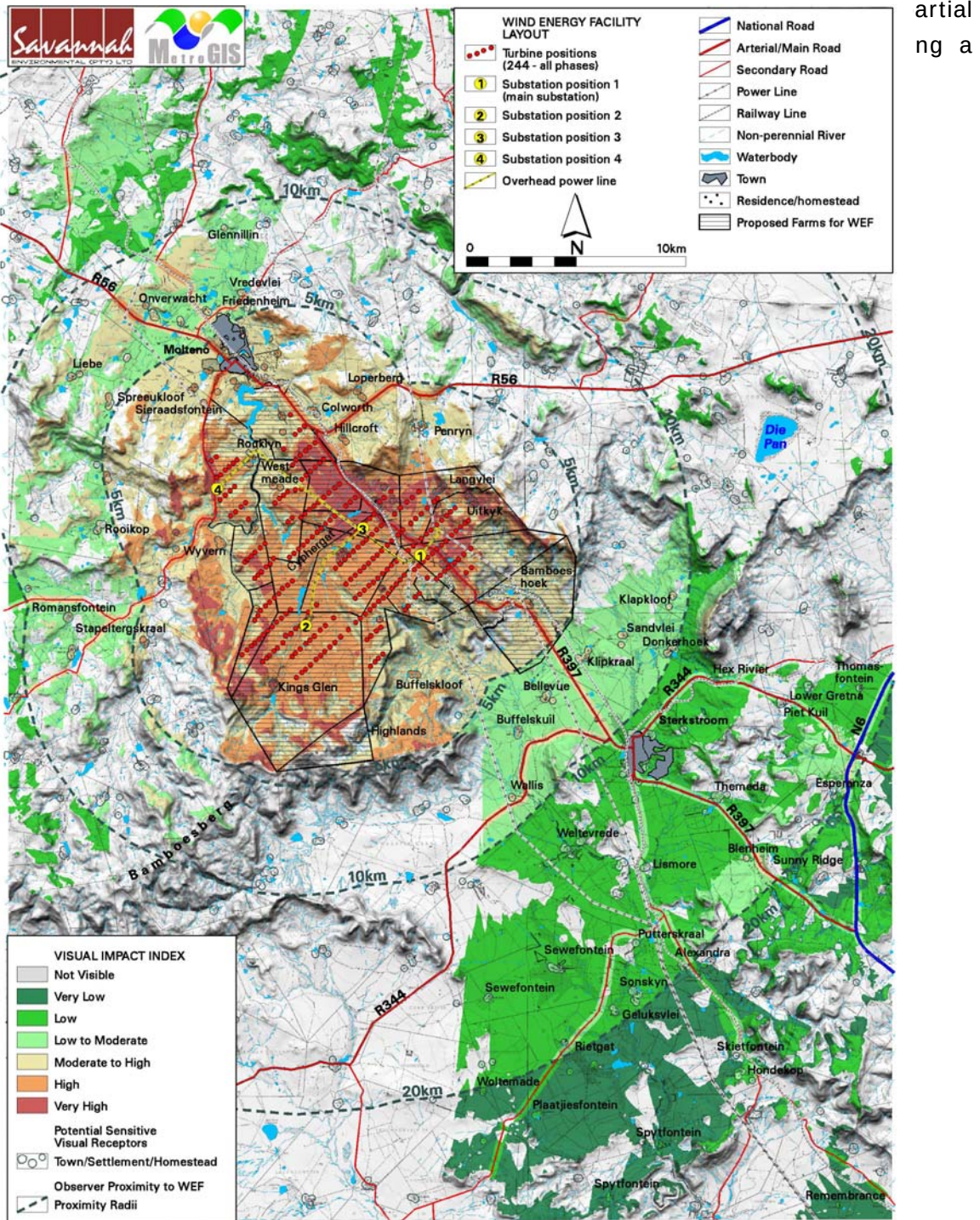
Figure 9.7: Visual impact index of the proposed Wind Energy Facility (all five phases)
