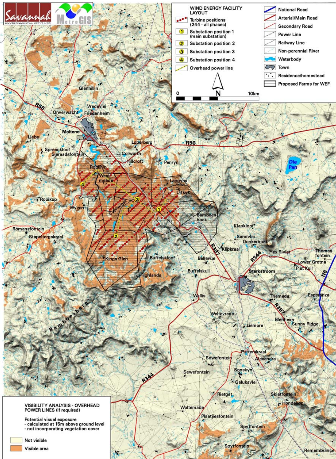
Figure 10.5 Potential visual exposure of the proposed power lines
