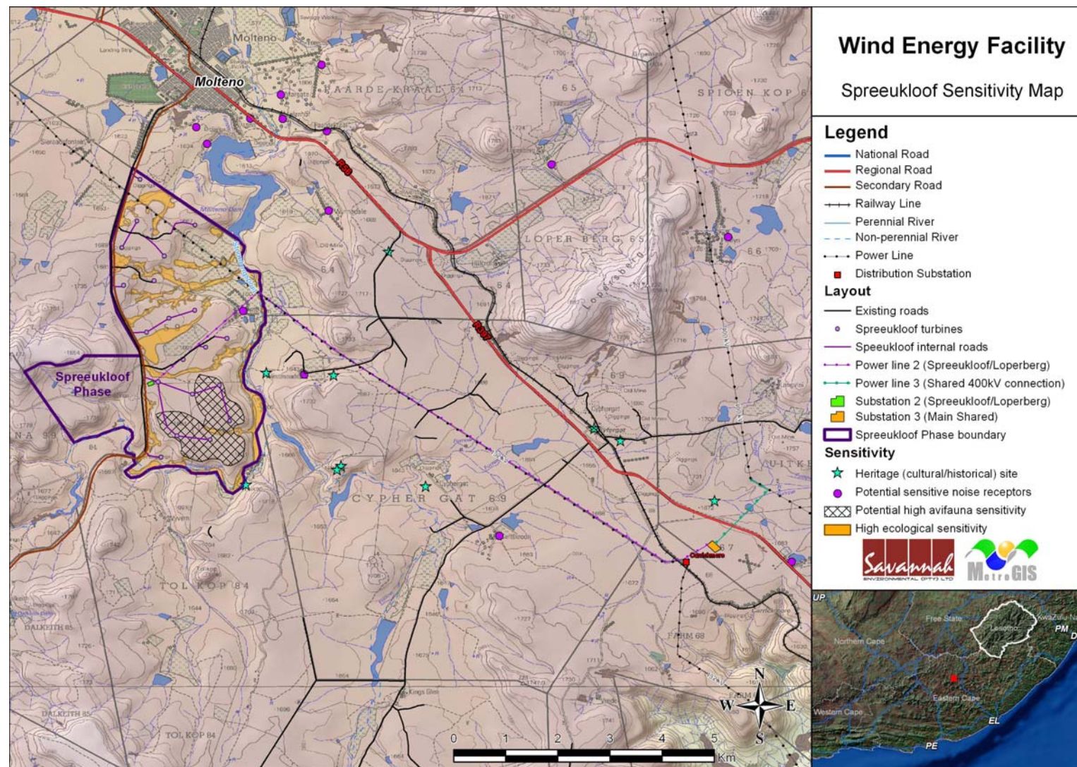
Figure 15.2: Combined sensitivity map for the Spreeukloof Wind Energy Facility project study area illustrating identified potentially sensitive areas in relation to the wind energy facility layout
