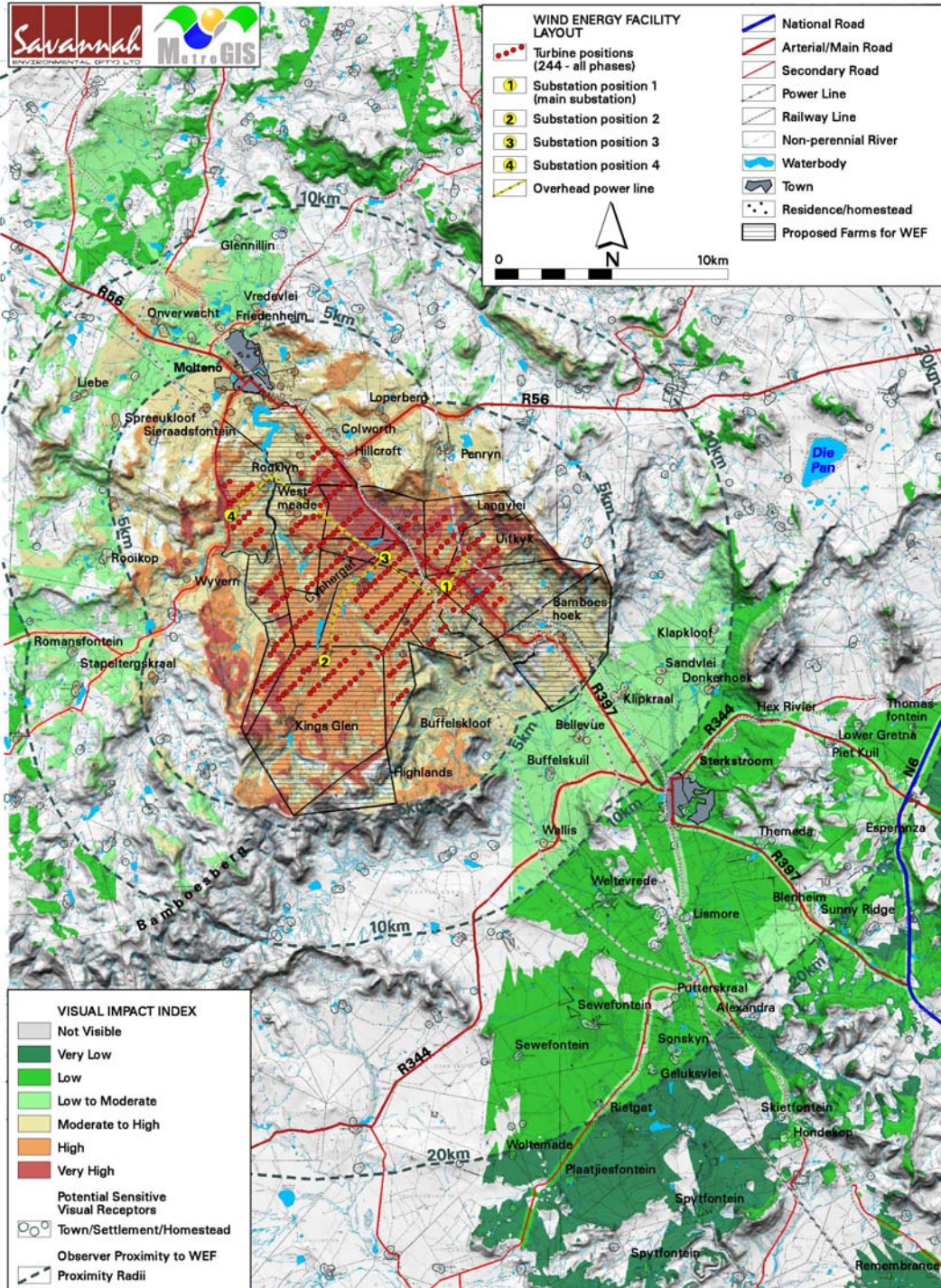
Figure 6.7: Visual impact index of the proposed Wind Energy Facility (all phases)
