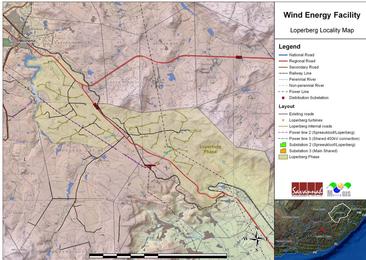
Figure 11.1: Map showing the proposed wind turbine layout, power line corridors and proposed substation sites for the Loperberg Wind Energy Facility
