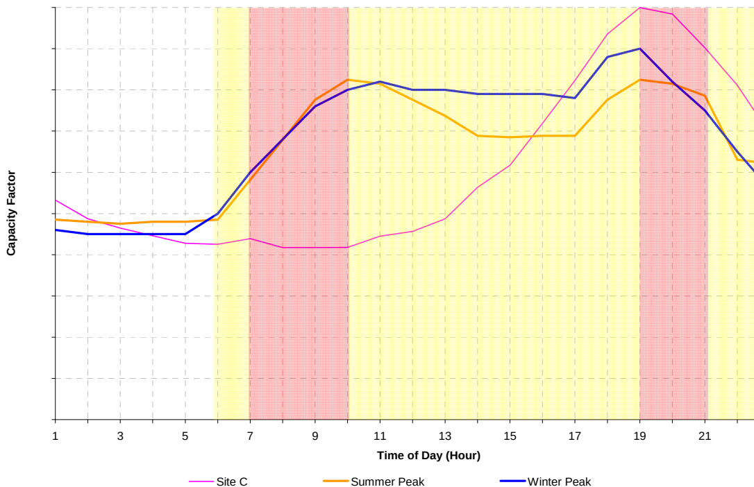
Figure 2.3. Load profile of a typical South African wind site. The graph shows an energy profile of a typical coastal site (pink line marked as Site C) where the overall energy yield is substantially lower than proposed site (i.e. for every turbine installed on the proposed site, more energy will be produced), even
