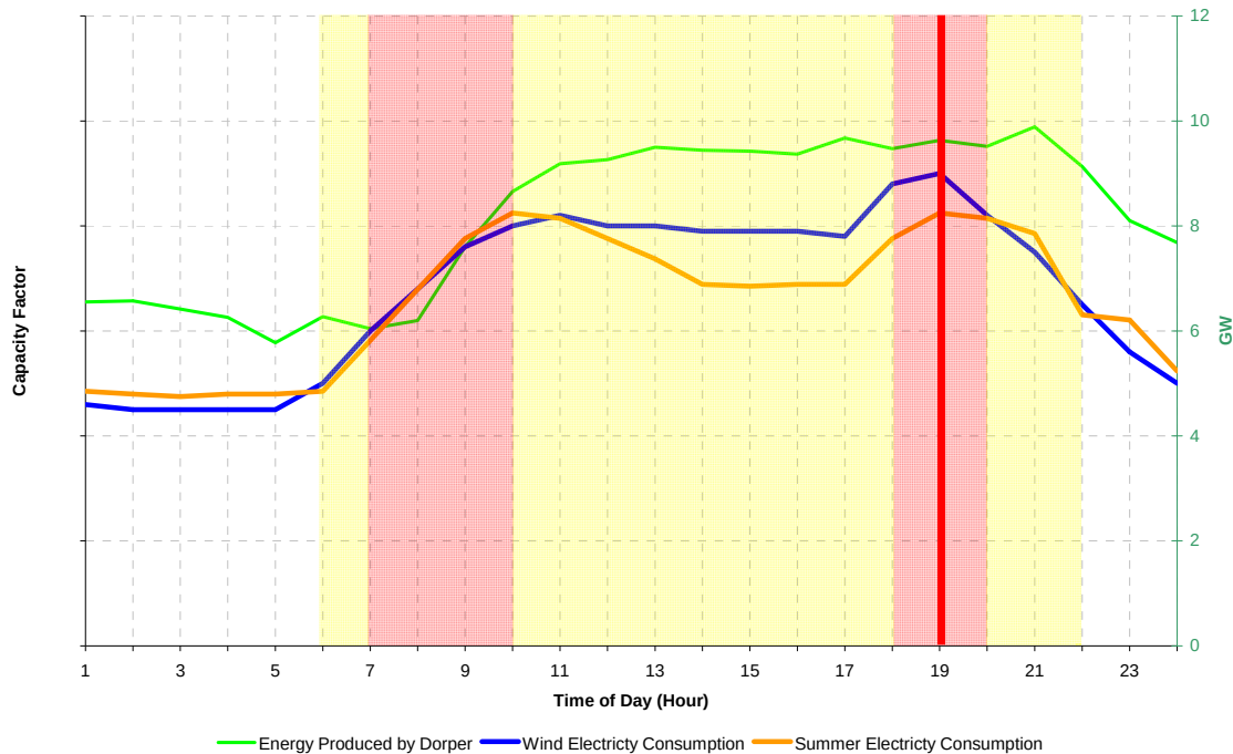
Figure 2.4. Energy produced by the proposed Wind Energy Facility. This graph shows the Energy Produced (Mean energy production) for the facility, as well as highlighting the energy production over winter. The profile matches the consumption pattern. Furthermore, winter production is extremely reliable and matches consumption. The colder South Africa's temperature, the higher the energy production, following consumption patterns where energy use increases during cold periods.
