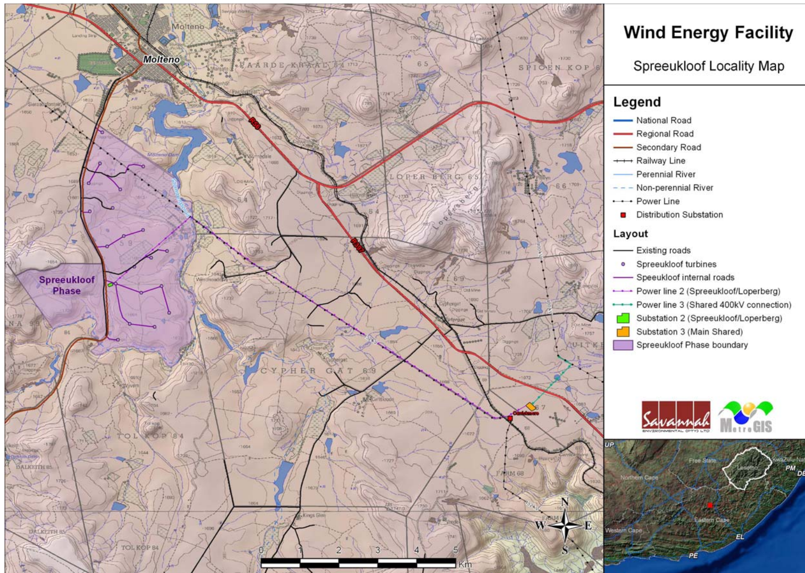
Figure 10.1: Locality map showing provisional wind turbine layout, power line corridors and substation sites
