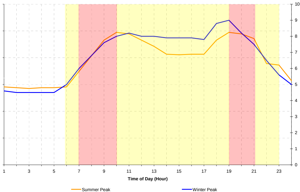
Figure 2.2. Load profile for South Africa, showing consumption during winter and summer periods. The Megaflex periods (red peak tariff, yellow standard tariff and white off-peak times) are overlaid onto this graph to further reinforce the value of electricity in South Africa at different times in the day. During the winter months, electricity as per the Megaflex tariff is double that of the summer tariff.
