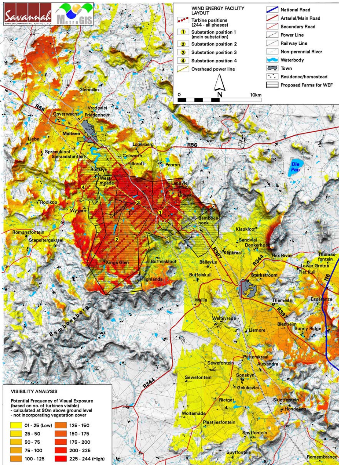
Figure 6.3 Potential visual exposure of the proposed wind turbines
