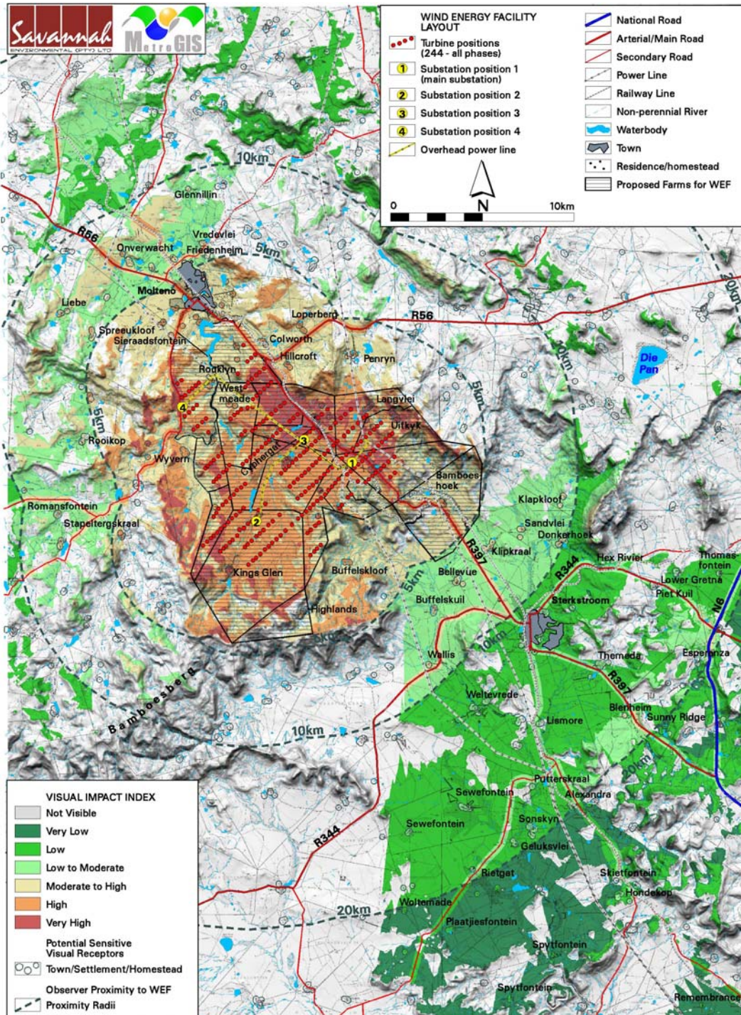
Figure 8.7: Visual impact index of the proposed Wind Energy Facility (all five phases)
