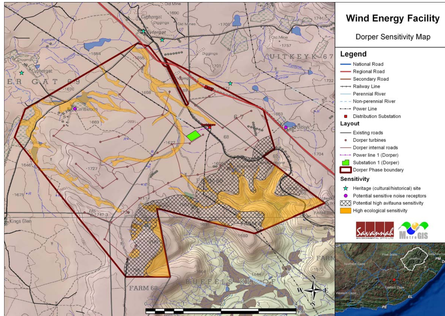
Figure 11.2: Combined sensitivity map for the Dorper Wind Energy Facility project study area illustrating identified potentially sensitive areas in relation to the wind energy facility layout
