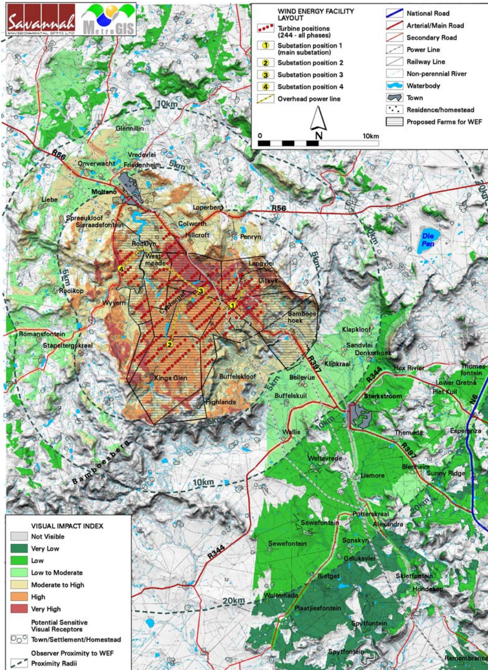
Figure 10.7: Visual impact index of the proposed Wind Energy Facility (all five phases)
