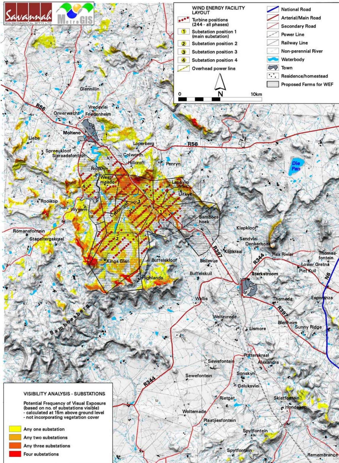
Figure 6.4 Potential visual exposure of the proposed substations
