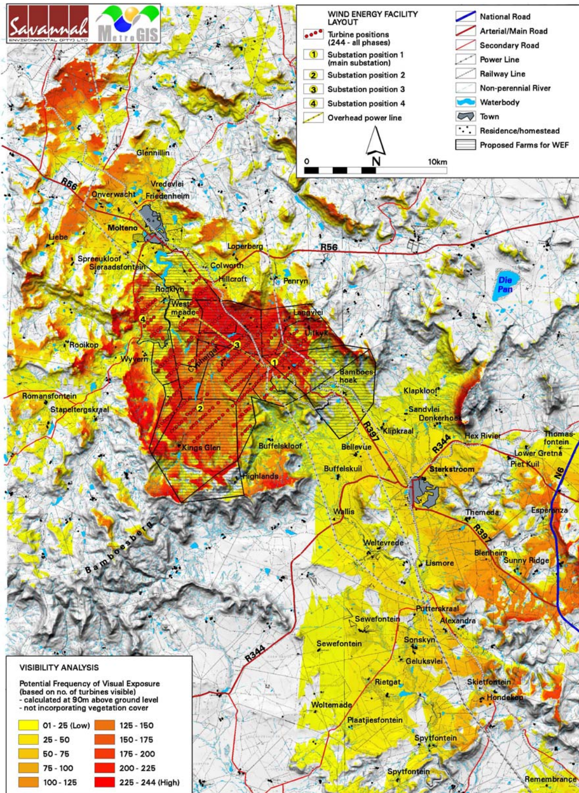
Figure 8.3 Potential visual exposure of the proposed wind turbines
