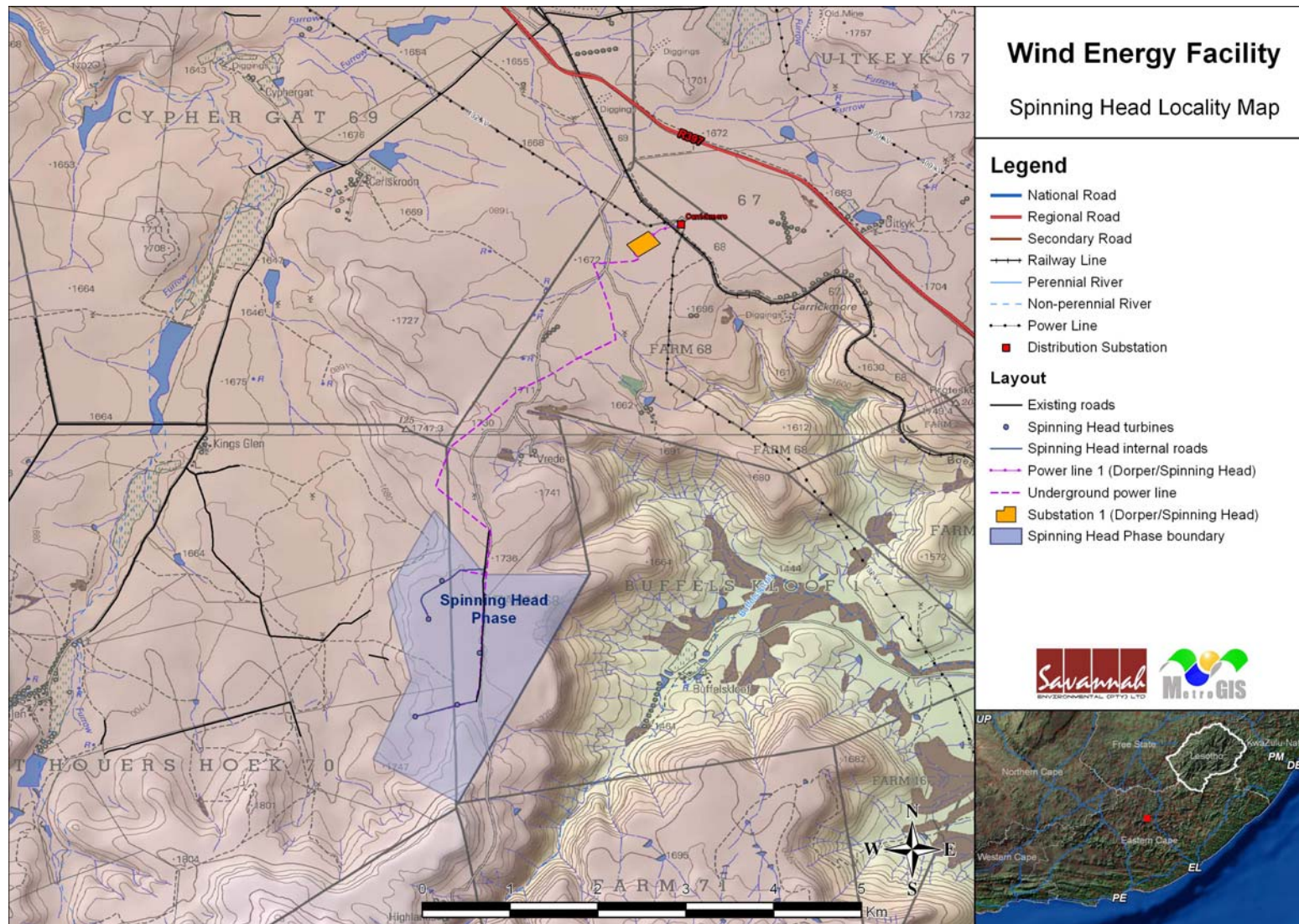
Figure 14.1: Map showing the proposed wind turbine layout, power line corridors and proposed substation sites for the proposed Spinning Head Wind Energy Facility
