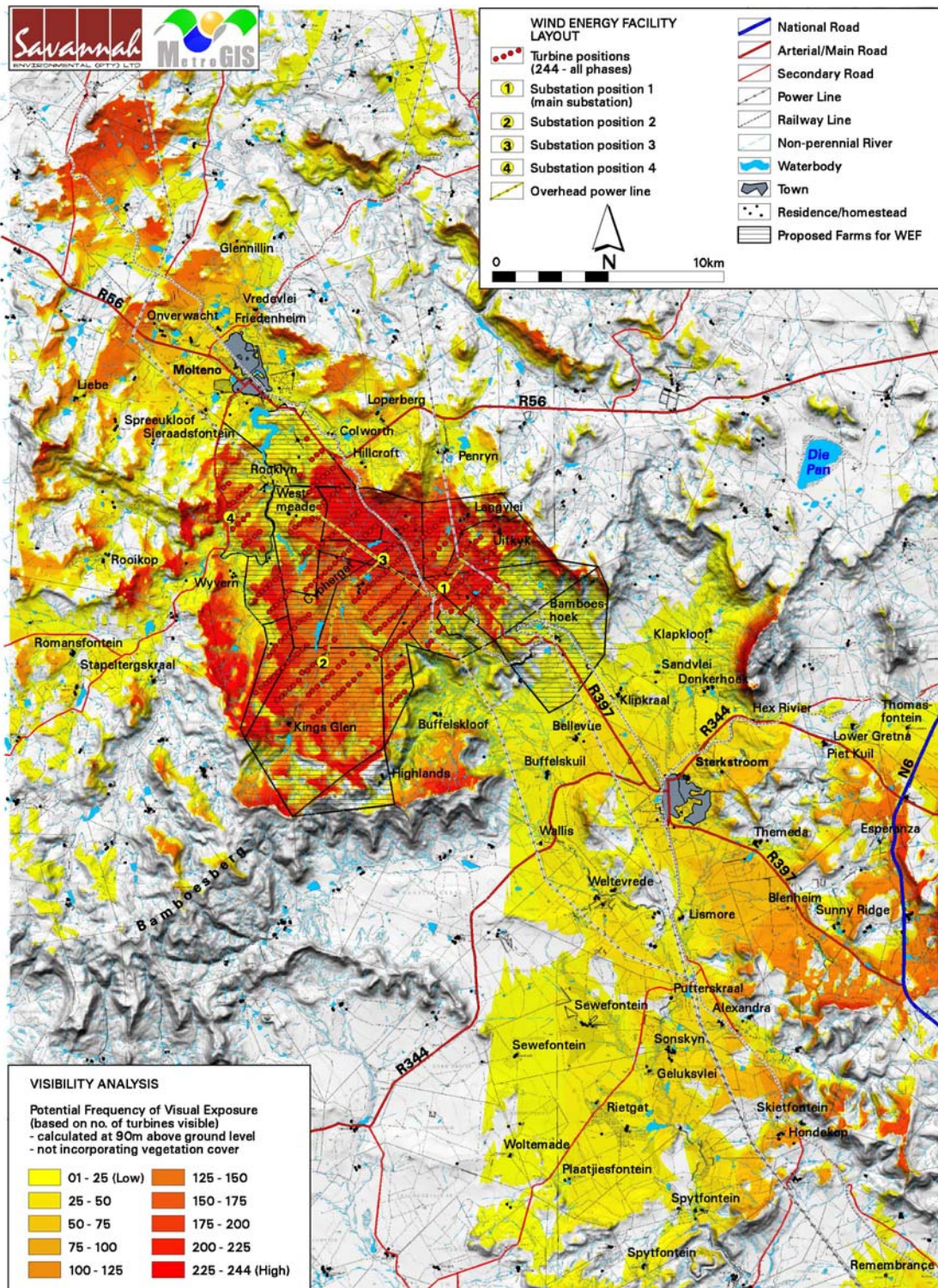
Figure 7.3 Potential visual exposure of the proposed wind turbines
