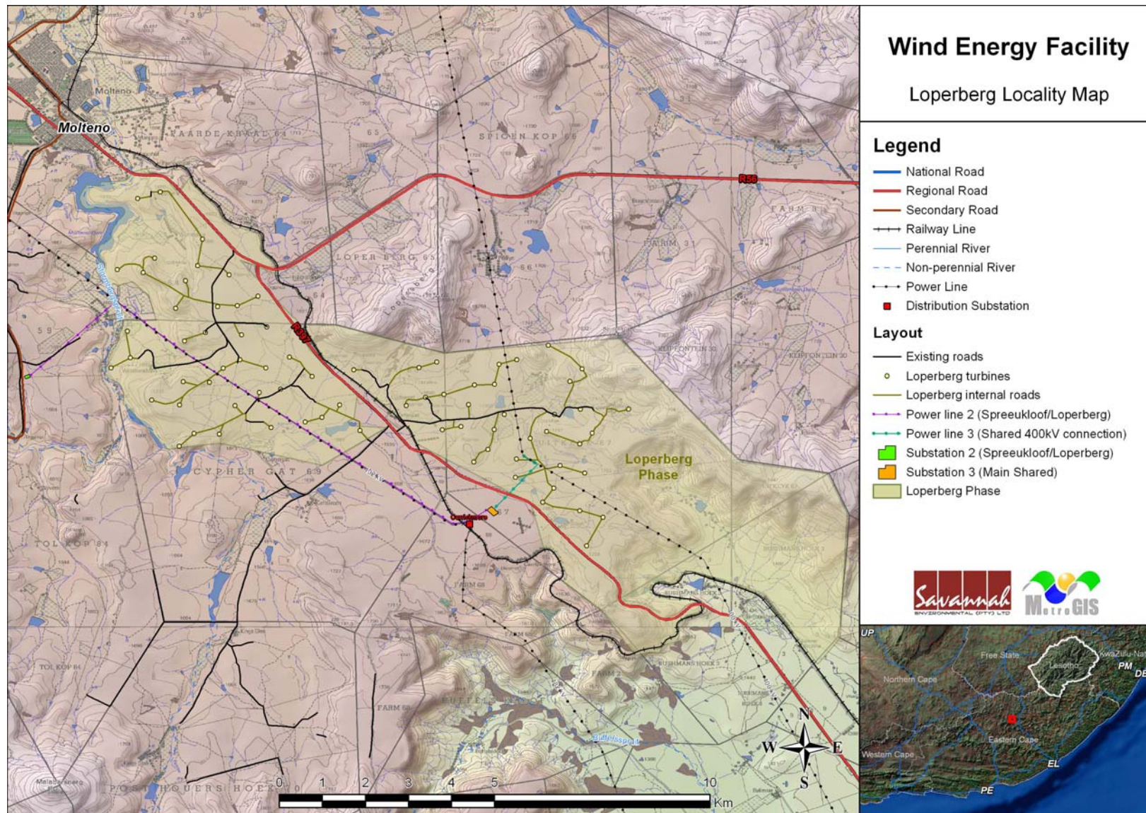
Figure 7.1: Locality map showing provisional wind turbine layout, power line corridors and substation sites
