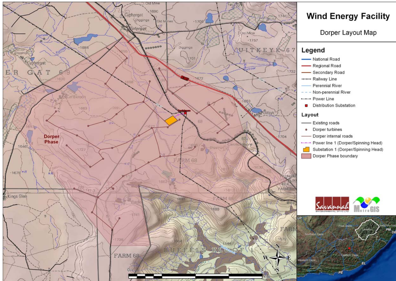
Figure 6.1: Locality map showing provisional wind turbine layout, power line corridors and substation sites
