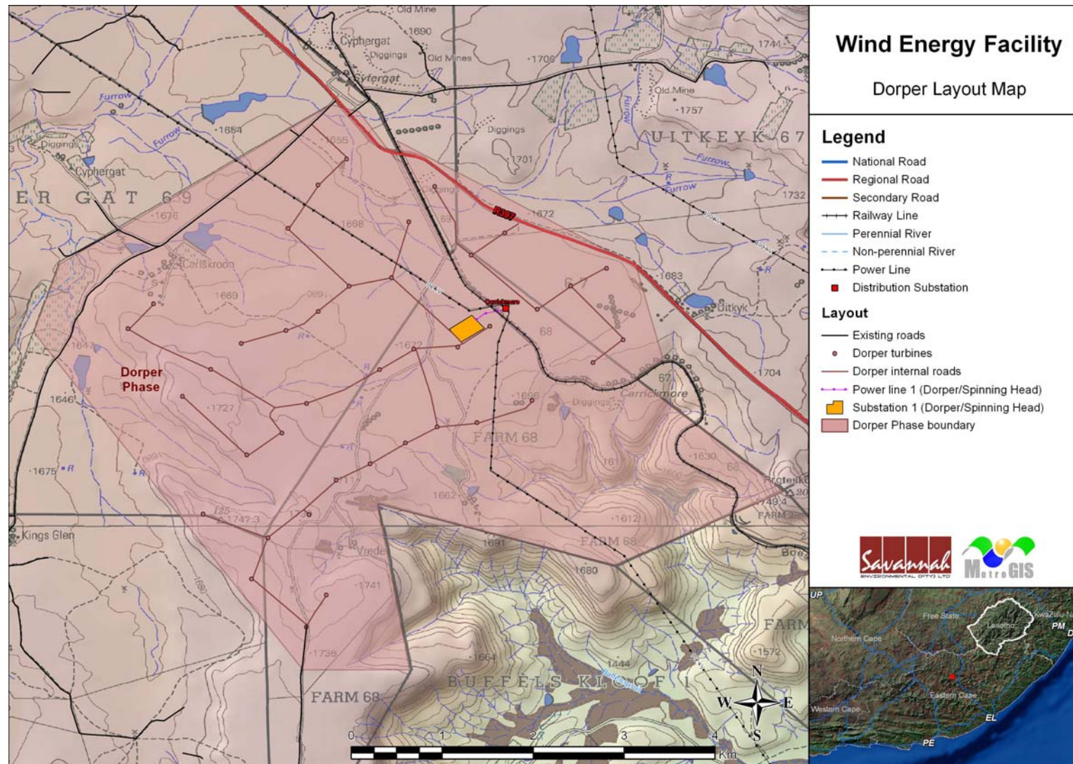
Figure 11.1: Map showing the proposed wind turbine layout, power line corridors and proposed substation sites for the Dorper Wind Energy Facility
