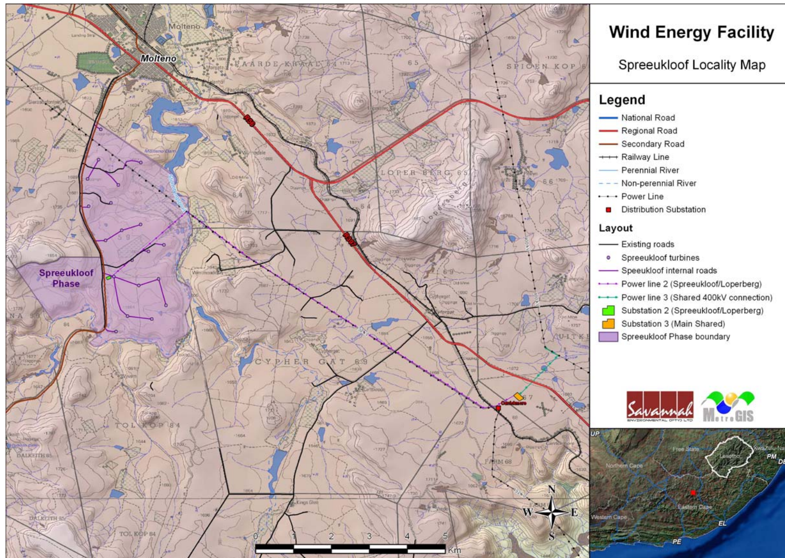
Figure 15.1: Map showing the proposed wind turbine layout, power line corridors and proposed substation sites for the proposed Spreeukloof Wind Energy Facility
