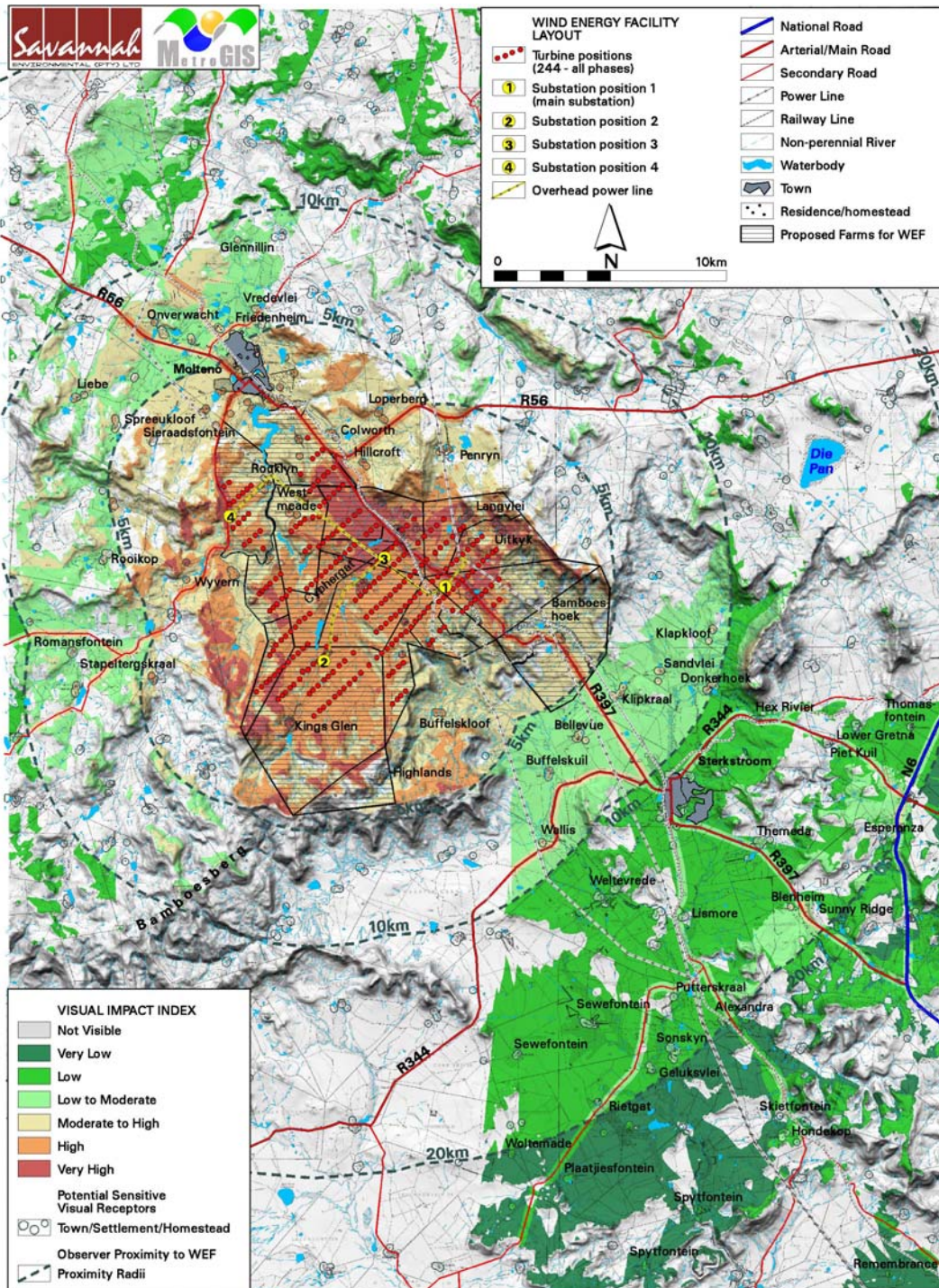
Figure 7.7: Visual impact index of the proposed Wind Energy Facility (all five phases)
