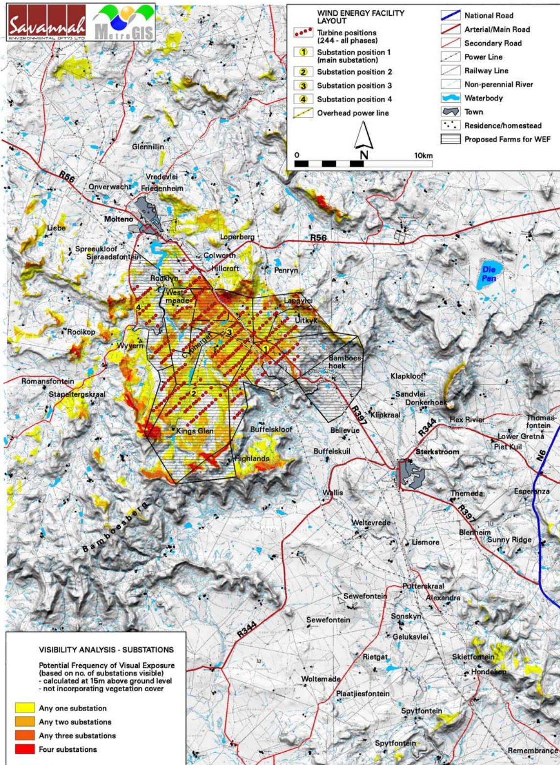
Figure 8.4 Potential visual exposure of the proposed substations
